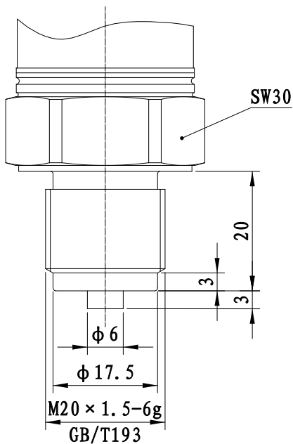
Process Connection (Code: M)
