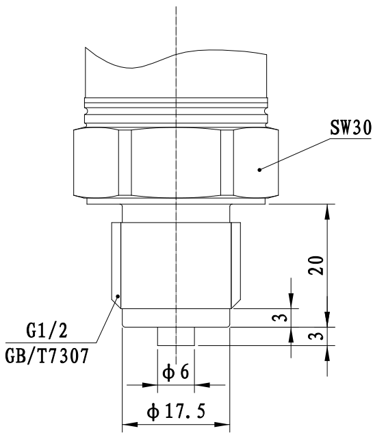
Process Connection (Code: G)
