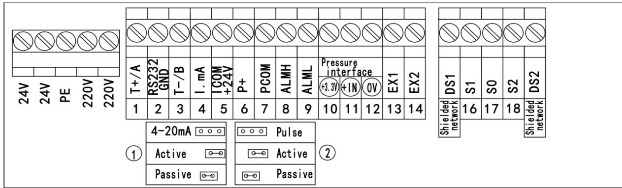
Figure 6 Remote Wiring
