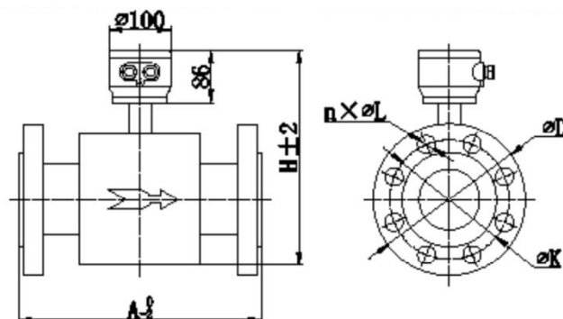
Figure 3 Remote Outline Dimensions
