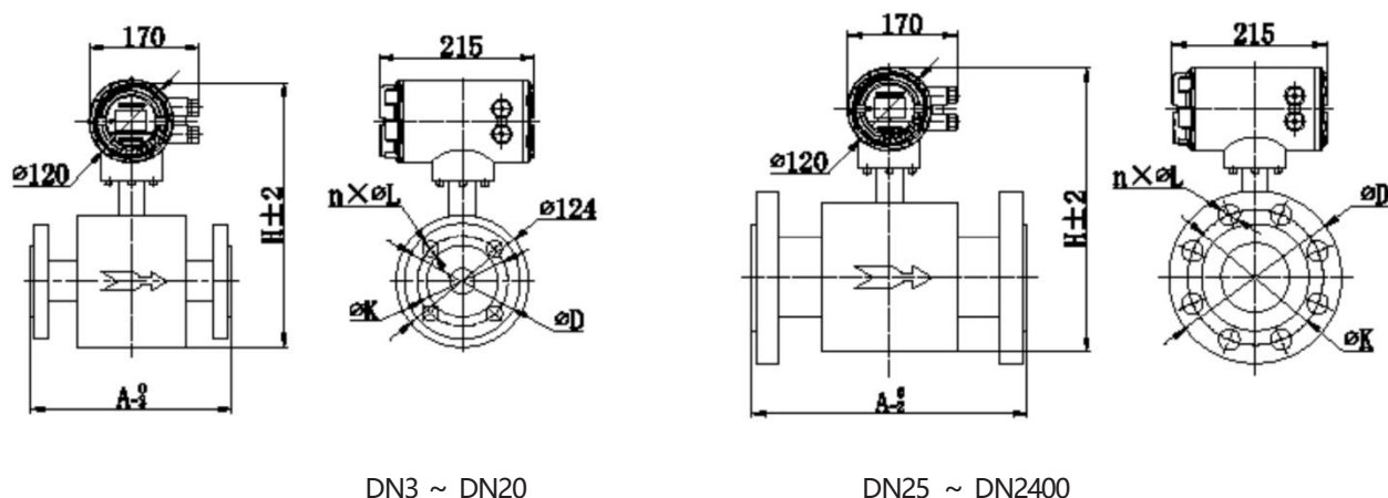
Figure 2 Integral Outline Dimensions
