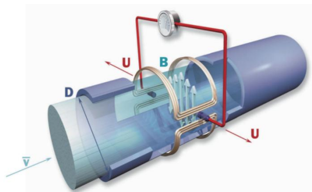
Figure 1 Operating Principle
