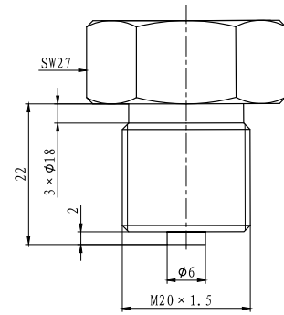
M20×1.5 Male, Waterline (C5)
