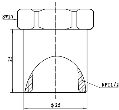
NPT1/2 Female (C11)
