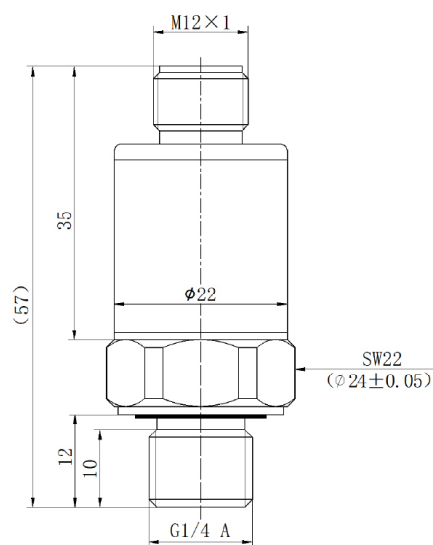
B4(M12x1 4-pin)
